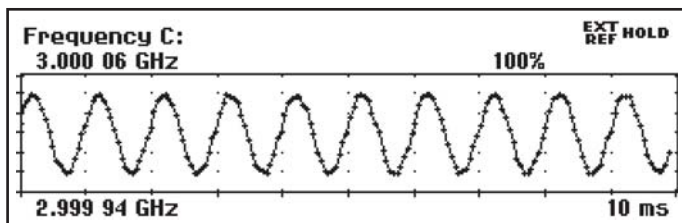
Figure 1: 1kHz FM with 12 ppm modulation depth
