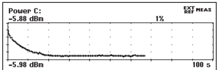
Figure 3: Generator start-up power settling
