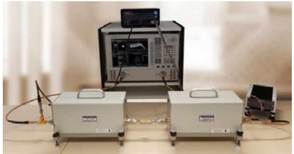
Pulsed DC and RF Load Pull bench architecture
