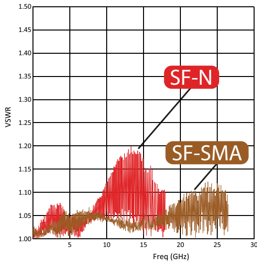
Maury StabilityFlex™ 36" Cable Assembly Typical VSWR
