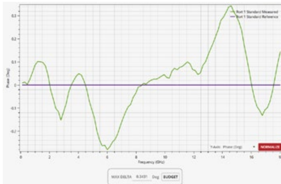
Figure 1. Normalized phase response between user-measured and factory-measured standard
